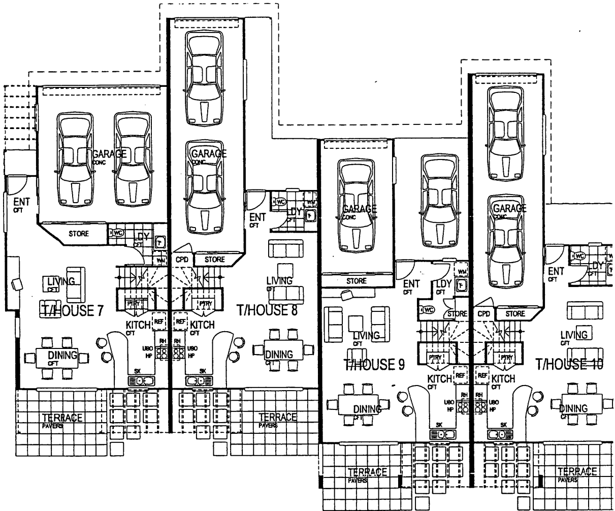
GROUND FLOOR PLAN CLUSTER 2: 3 BEDROOM TOWNHOUSES 1:100
